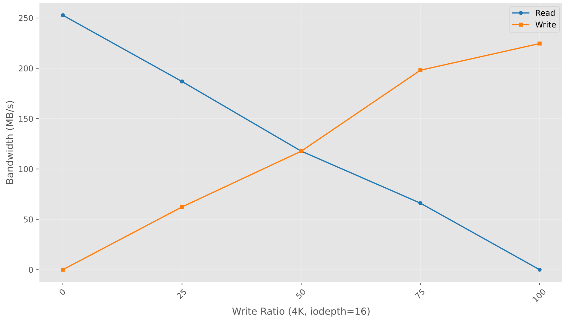
Bandwidth vs Write Ratio (4K, iodepth=16)
